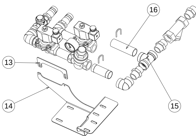
单进水管路 Single water inlet pipe assembly
