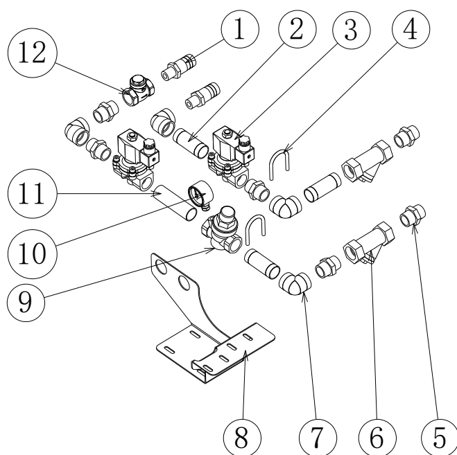
双进水管路 Double water inlet pipe assembly
